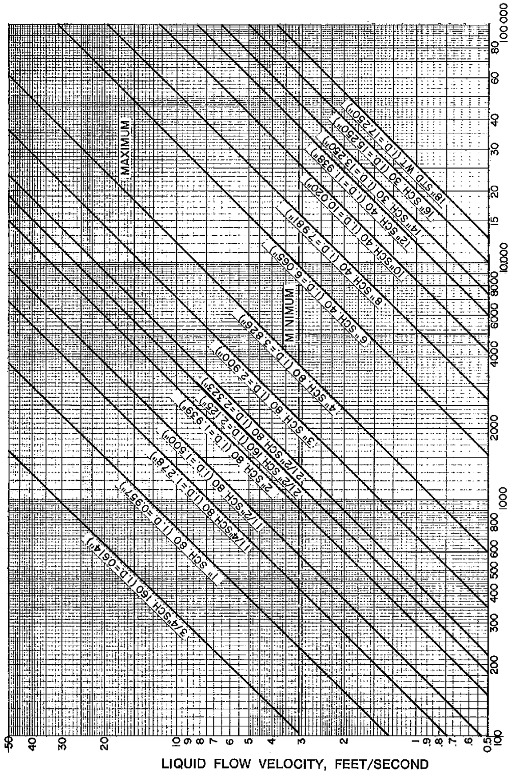
LIQUID FLOW RATE, BARRELS FLUID/DAY
