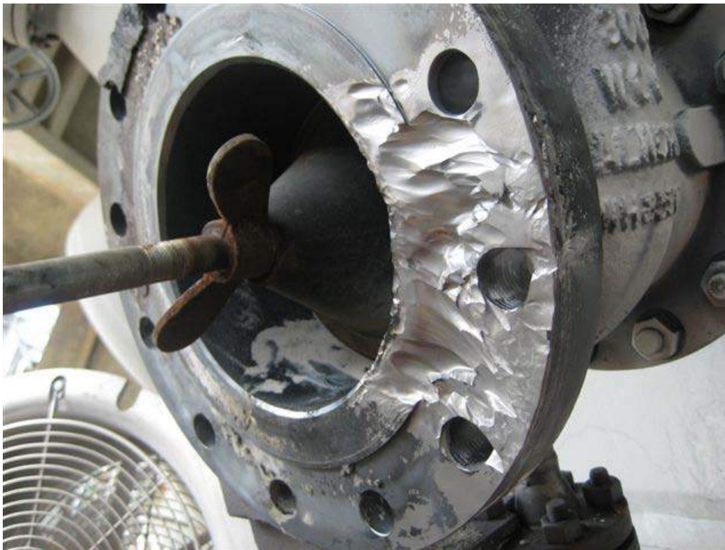
Figure 4-43 – Erosion Corrosion of a 1.25Cr 300 # valve flange on an FCC Catalyst withdrawal line.
