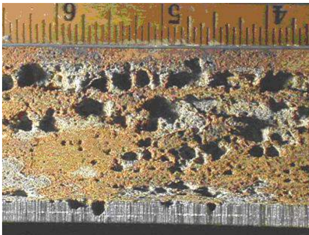
Figure 4-86 – Higher magnification view of the corrosion pits in Figure 4-85.
