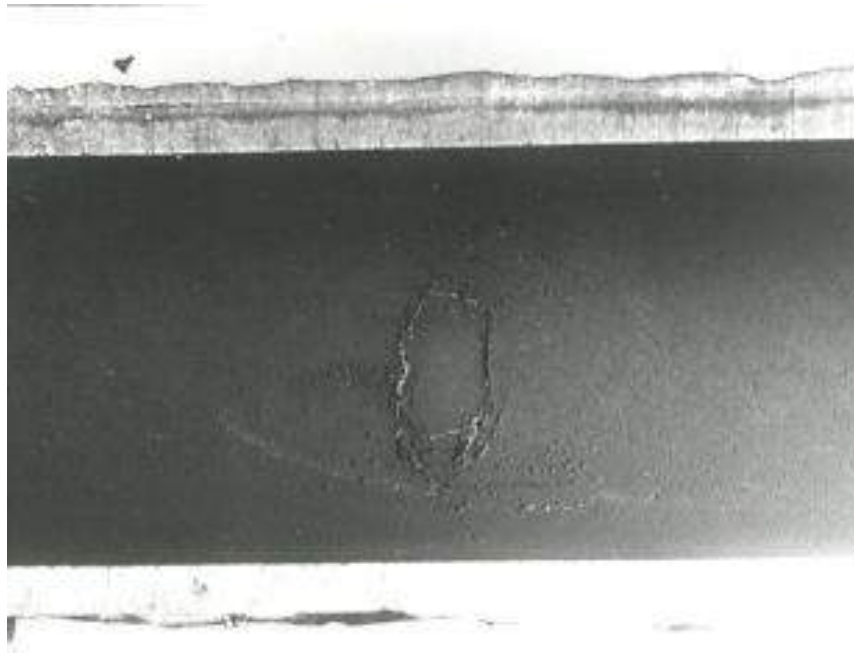
Figure 4-144 – Photograph of a carbon steel boiler tube cut in half lengthwise. Corrosion fatigue cracks initiate at the I.D. of a tube, opposite a buckstay attachment on the O.D. (Mag. 1X)
