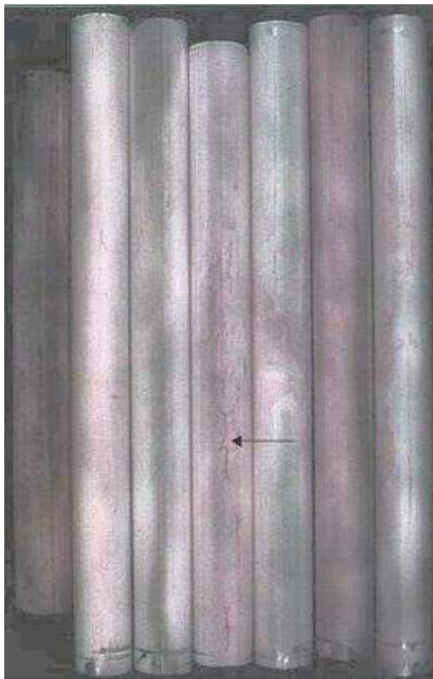
Figure 4-135 – Cracking on the shell side of Type 316L SS tubes in steam service at 450°F (232°C), showing tubes after PT inspection. The cracks can be seen in the center tube (arrow).
